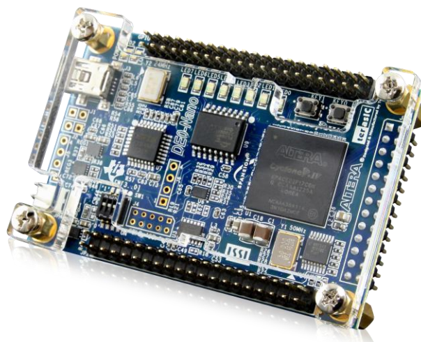
Figure 1-1 The DE0-Nano Board
