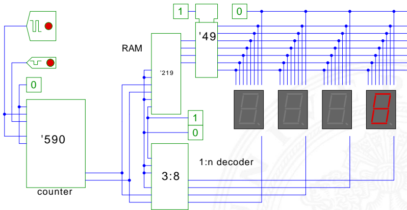
7-segment decoder
