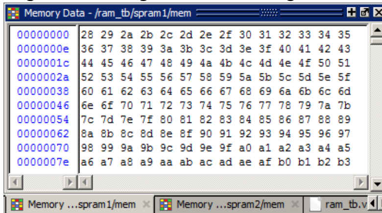
Figure 7-4. Verilog Data After Running Simulation
