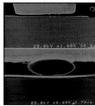
Figure 4 Cross-sectional view of interconnection by a 2-µm-diameter electrically conductive particle for the TCP and an aluminum-beryllium electrode on the glass panel.
