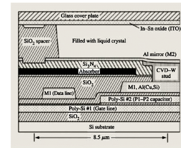
Figure 1 Schematic cross section of a pixel of the four-million-pixel light valve.
