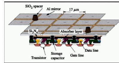
Figure 1 Schematic diagram of a spatial light-modulator array showing the cross section of the light valve used in the prototype monitor. To complete the light valve, a top glass plate with a transparent conductive layer is placed on top of the posts and glued to the silicon substrate along the edges. Finally, the gap between the mirrors and glass is filled with liquid crystal material.
