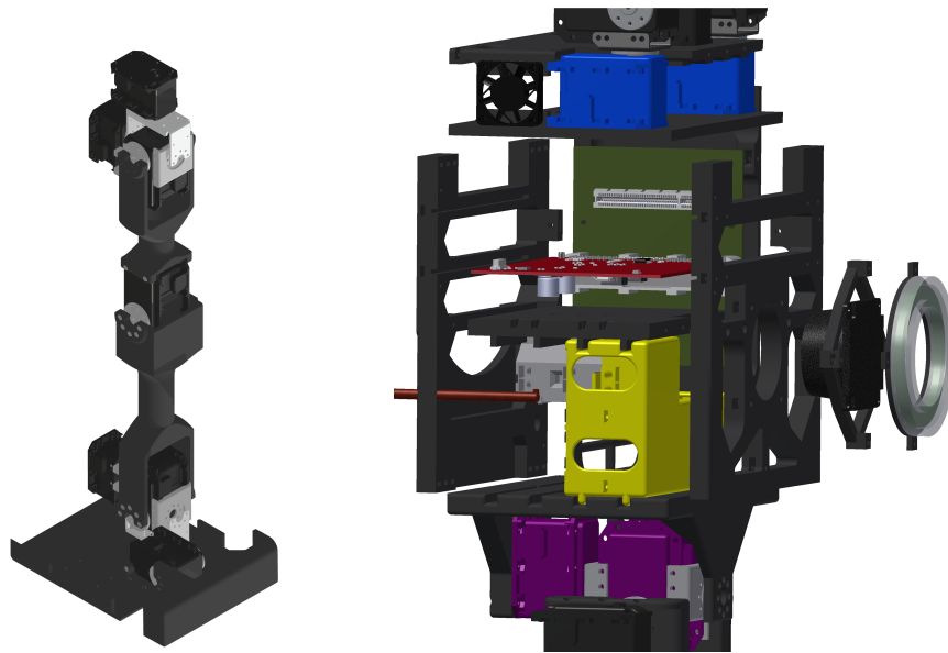
Fig. 2: CAD model of the leg ( left ) and explosion view of the torso ( right ). Note the additional shoulder servos (blue) and the new waist joint (purple). The two batteries (yellow, only one shown) are inserted from the left and locked by a bolt (brown) which fits into a bayonet socket. The powerboard (red) and motor controller board (not shown) are directly plugged into the backbone board (green) and locked by a side plate (not shown).
