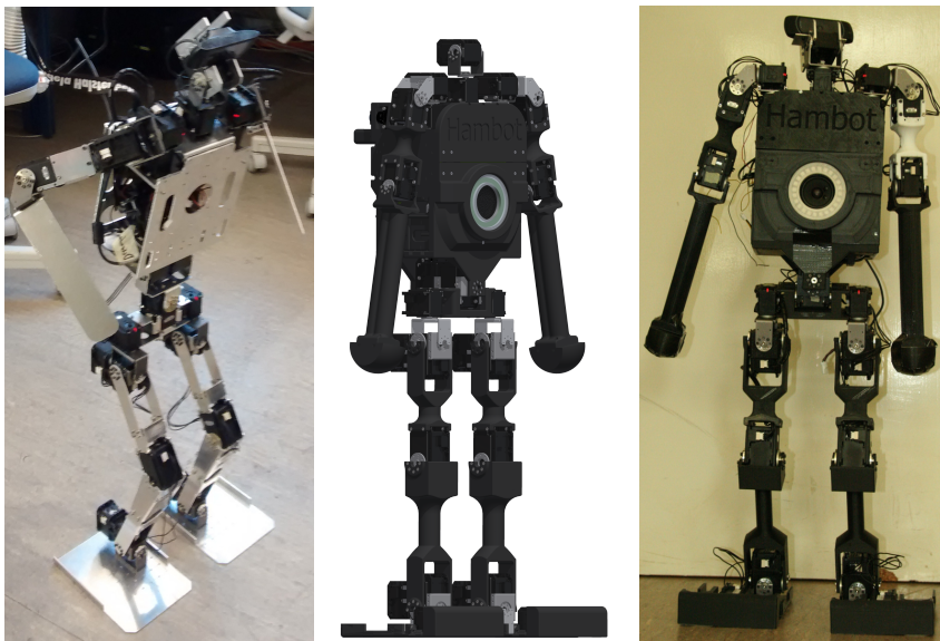
Fig. 1: Prototypes of GOAL ( left ) and Hambot ( right ). CAD model ( center ).
