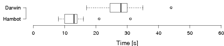
Fig. 3: Time for battery change, tested by a group of trained and untrained test persons. Median time: Darwin 28s, Hambot 13s.
